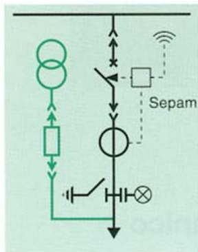
Salida LF-B, TF-B, MF-B, CB-B
