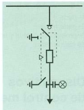
Salida inter fusibles TF-S
